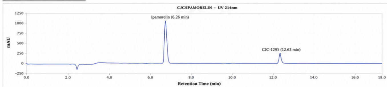
CJC/IPAMORELIN 10mg - NL-CJ05261: UV Chromatogram
