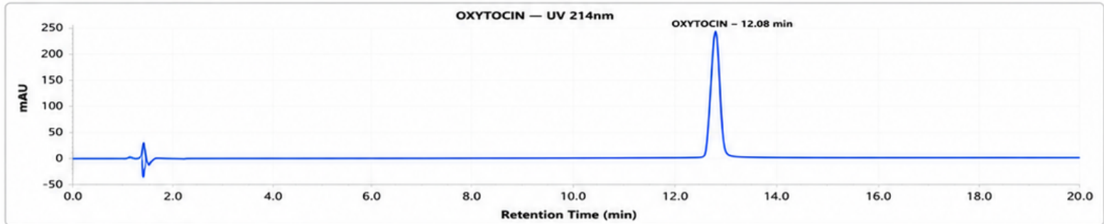
OXYTOCIN 10mg - PS-OXY05261 : UV Chromatogram
