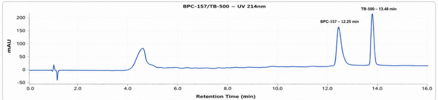
BPC-157/TB-500 10mg – PS-W05261 : UV Chromatogram
