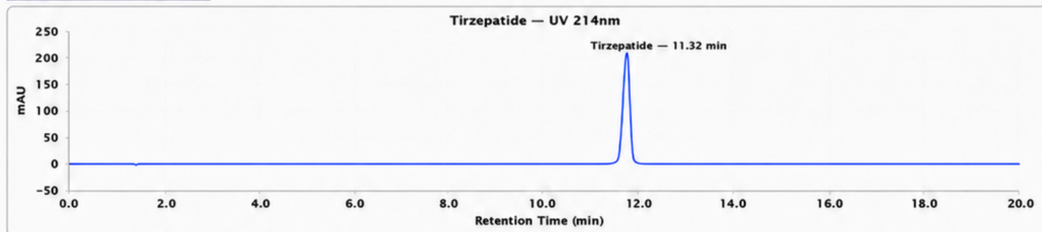
Tirzepatide 30mg - PS-TIRZ150005261 : UV Chromatogram
