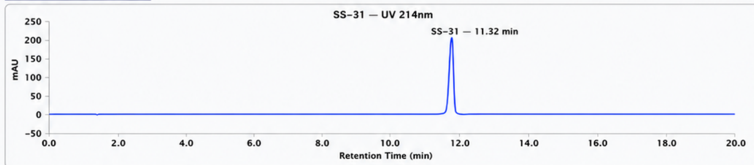
SS-31 10mg - PS-TIRZ150005261 : UV Chromatogram
